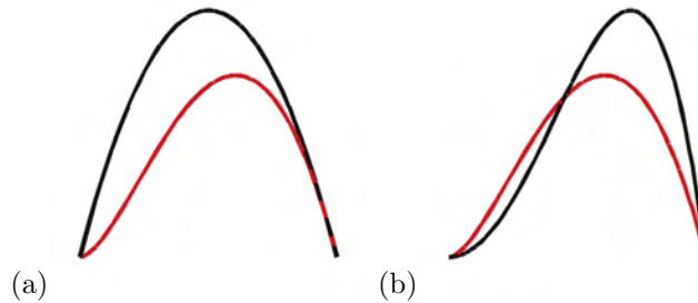
Figure 1.2. Graphical comparison of y - y^2 and y^2 - y^4 to -y^2 \log(y) (red)
