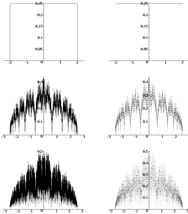
Figure 5.10. 26th iterate for q = 1/2 (top), q = 0.6 (middle) and q = (\sqrt{5}-1)/2 (bottom).
