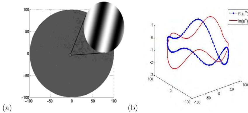
Figure 4.1. (a) Real part of incident field with direction \hat{\eta} = -\pi/12 , and wavenumber \kappa = 2 on the domain \mathbb{D} . The inset is a close-up view of the field. (b) Far field data, real and imaginary parts, corresponding to scattering due to the passing of the incident plane wave shown in (a) through the domain \mathbb{D} .
