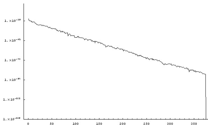
Figure 2.1. Smallest entry of y_k = A_k^{-1}x in a typical PSLQ run, as a function of k .
