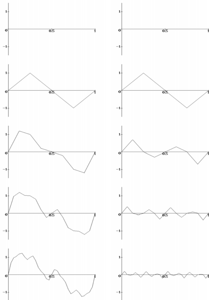
Figure 5.4. Piecewise affine approximations to the Weierstrass function S_{1/2,2} .
