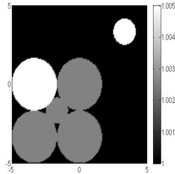
Figure 4.6. The true scatterer consisting of 6 circles of different sizes and indices of refraction indicated by the color.
