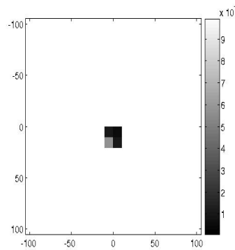
Figure 4.3. Plotted is the value of the integral in (4.51) at the reference points z \in \mathbb{D} where \mathbb{D} is shown in Figure 4.1(a). The test domain \Omega_t is a circle of radius t = 5\sqrt{2} and with a cutoff value in (4.51) of M = 9 . If proposition 4.8 is true, then the scatterer lies in the region \mathbb{G} + \Omega_t where \mathbb{G} is the set of points in the dark region above.
