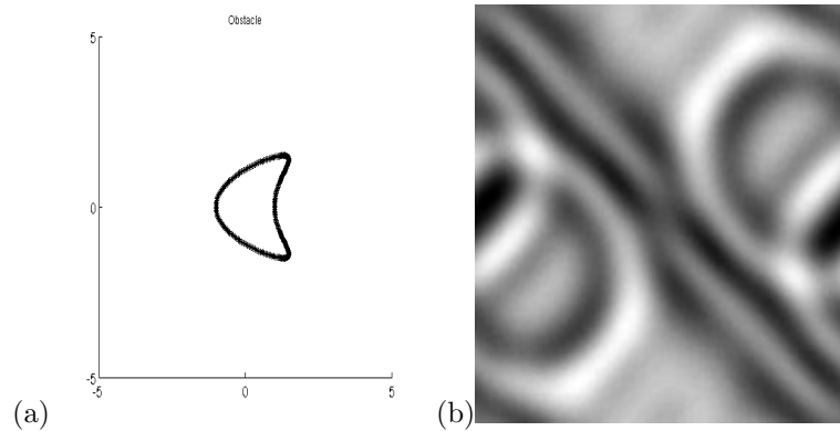
Figure 9.1. (a) Kite-shaped obstacle given by (9.48) and generated by the Matlab code in section 5.1 of Chapter 4. (b) Real part of far field data for Exercise 8. Partial code for generating this data is given in section 5.2 of Chapter 4.
