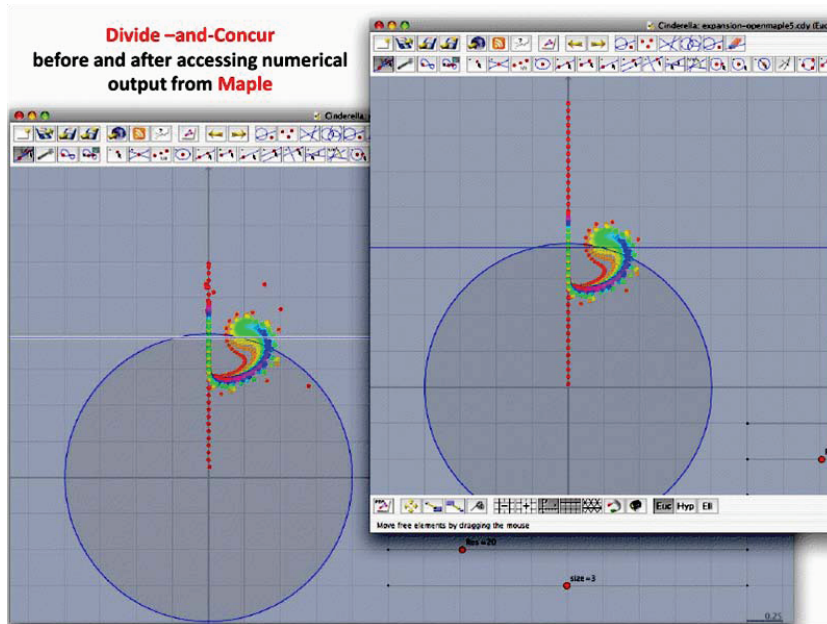
Figure 8: Multiple iterations in Cinderella.
