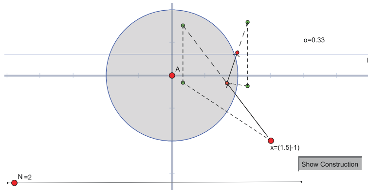
Figure 1: Two steps showing the construction.
