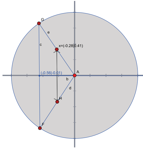
Figure 3: Iterated reflection with a ray.
