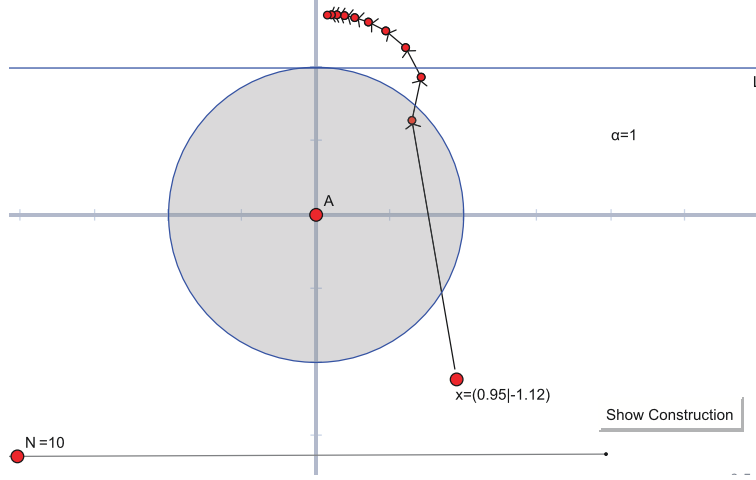
Figure 7: Case with \alpha = 1 .
