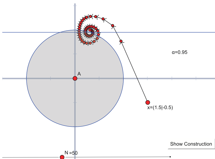
Figure 5: Case with \alpha = 0.95 .
