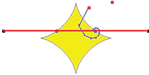
Figure 9: Spiralling with the 1/2-sphere.
