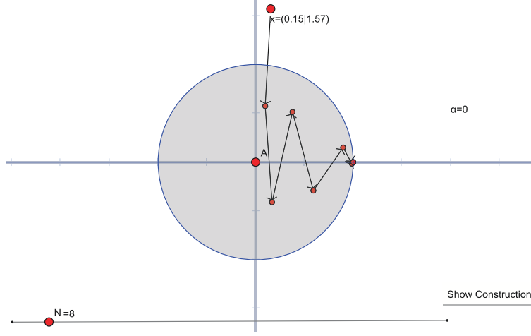
Figure 6: Case with \alpha = 0 .
