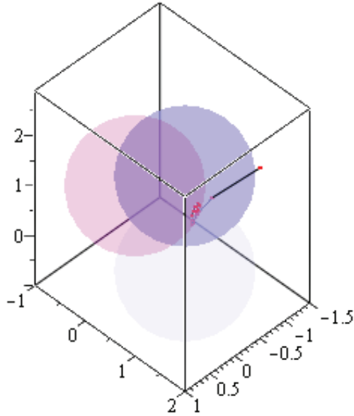
Figure 2: Douglas-Rachford for three spheres in three-space.
