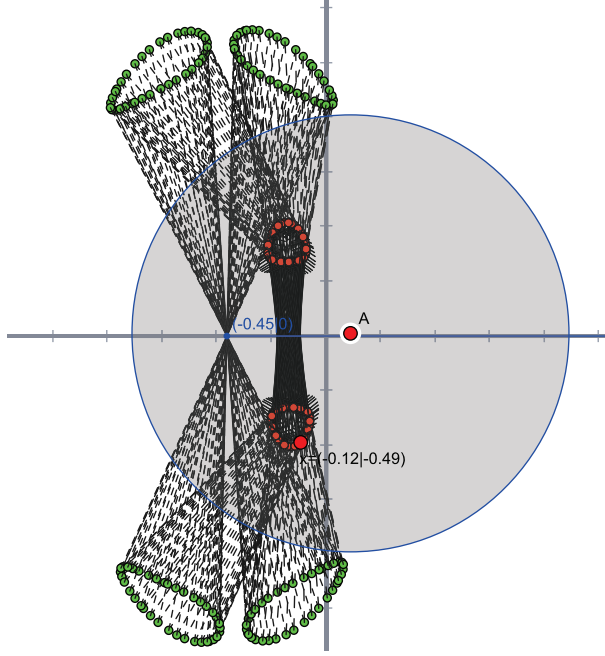
Figure 4: More complex behaviour for a ray and circle.
